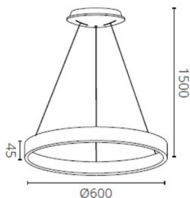
LOOP 60
